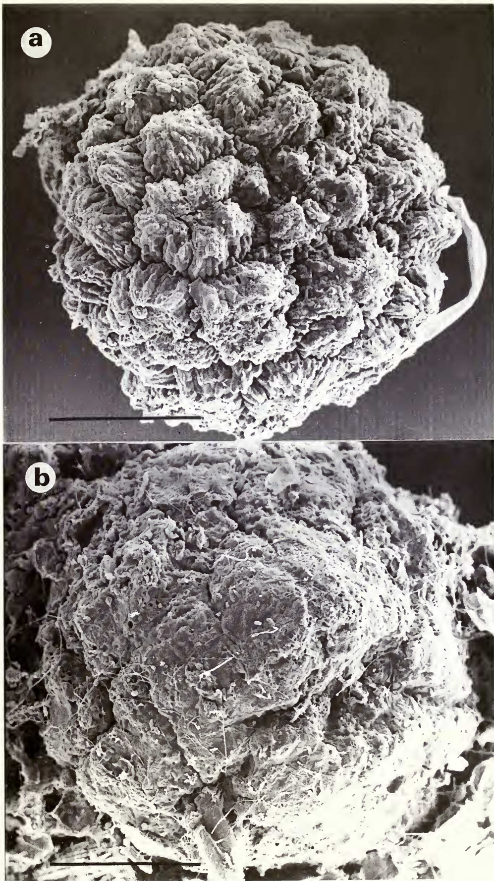
Fig. 57 Rhytidiella moriformis Zalasky (IMI 136514) (a) Surface view of ascoma; scale = 136 \mu m. Rhytidiella beloniza (Stirton) Aguirre (BM-isotype): (b) Surface view of ascoma; scale = 120 \mu m.
